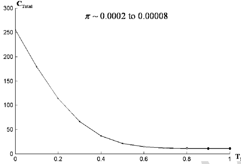
Fig. 5. Minimum Cost Curves for Series System.
