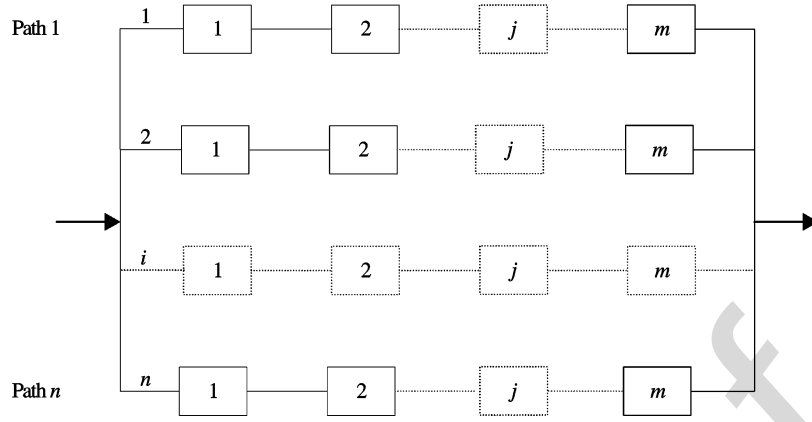
Fig. 1. Conceptual Depiction of Parallel-Series System.
