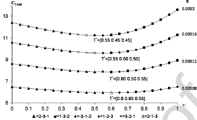
Fig. 4. Minimum Cost Curves for Parallel System.
