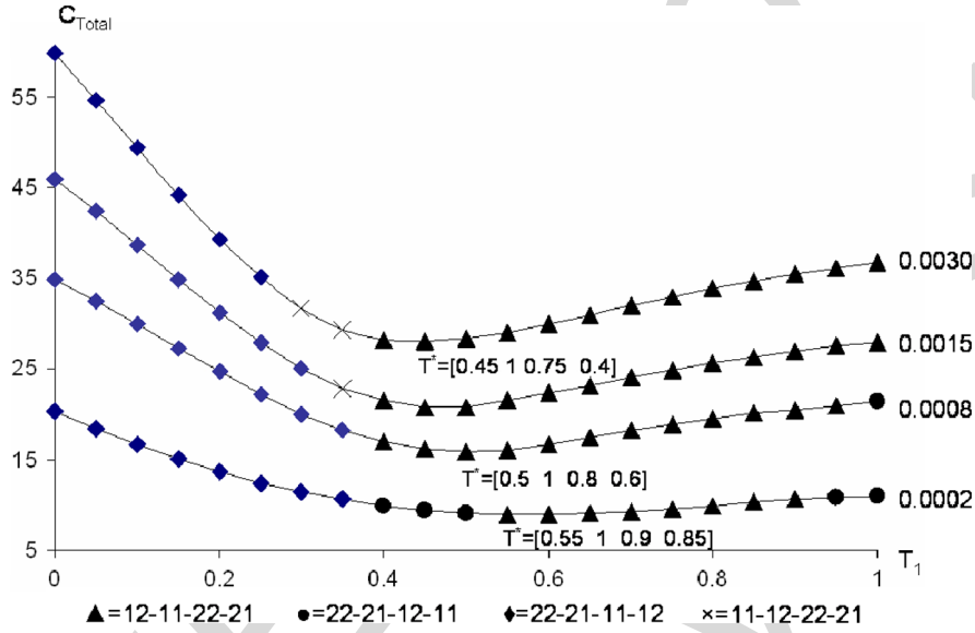
Fig. 6. Minimum Cost Curves for Parallel-Series System.
