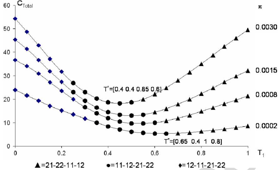
Fig. 7. Minimum Cost Curves for Series-Parallel System.
