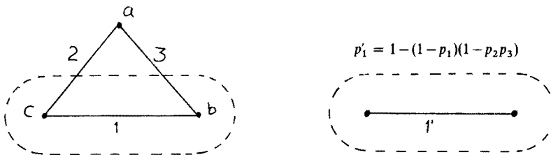
Fig. 1.1. Reduction of series-parallel communication network.
