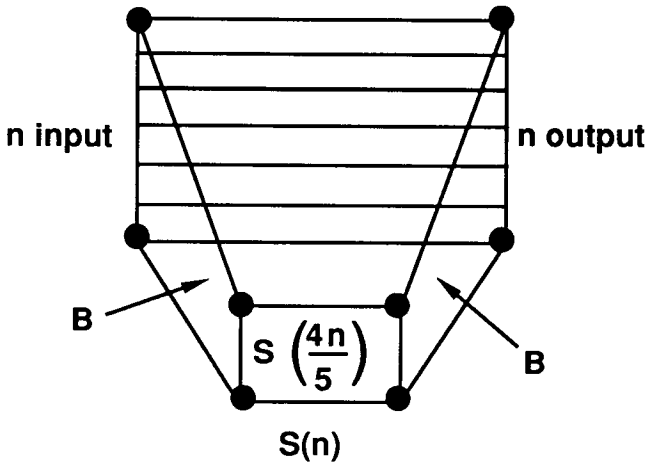
Figure 3: a superconcentrator
