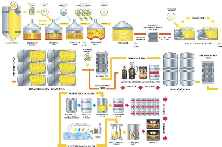
Figure 1: Diagram of brewing. Source: Brewery Svijany.
