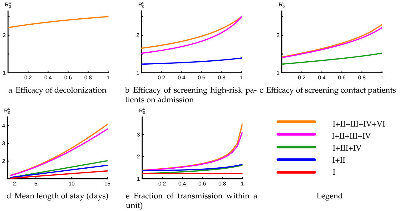
Fig. 10. Changes in critical transmission parameters ( R_0^c ) for different combinations of intervention measures according to changes in model parameters. Default values of the parameter are shown in Table 1.
