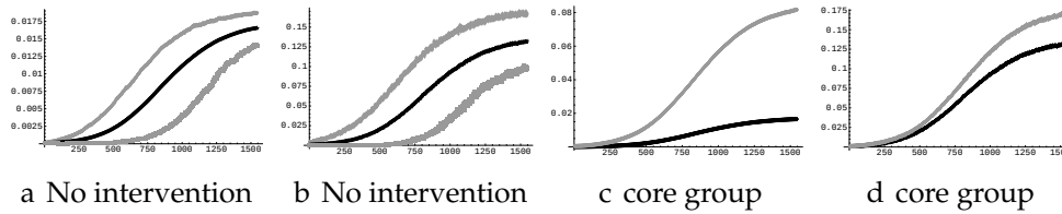
Fig. 7. Simulations without intervention measures and an initial low prevalence. (a) Prevalence in the population. (b) Prevalence in the hospitals. The black lines indicate the average behaviour of a hospital. 90% of the simulations fall between the grey lines (c) Mean prevalence in the extramural population, the black line for the total extramural population, the grey one for the core group population (d) Mean prevalence within the hospitals, the black line for the total intramural population, the grey one for the intramural core group population
